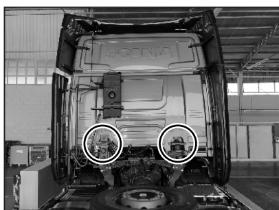
Area where the mount must be installed, passenger side.
